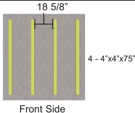
Front Side Gravel Foundation with treated stringers
